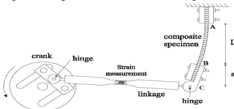
Fig.2. Schematic line diagram of Hinge Eccentricity, Load Cell and Specimen Holding Arrangement
