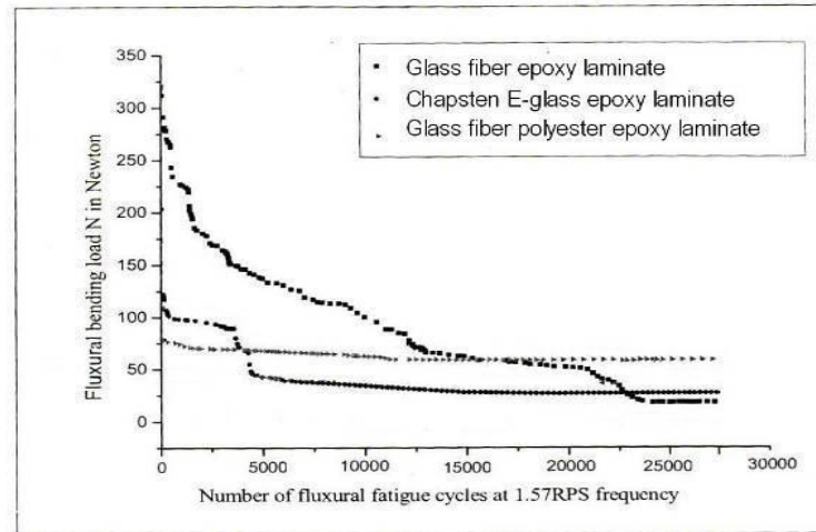
Fig. 12.3. Consolidated Flexural Fatigue Test Results of Glass Fiber Epoxy, Chapsten E-Glass Epoxy and Glass Fiber Polyester Epoxy laminates.
