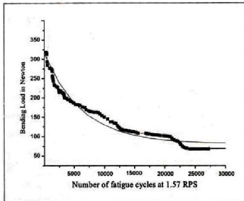
Fig. 11.1 Stiffness Degradation behaviour of Glass Fiber Epoxy laminate Number of Fatigue Cycles at 1.57 RPS for Glass Fiber Epoxy Laminate
