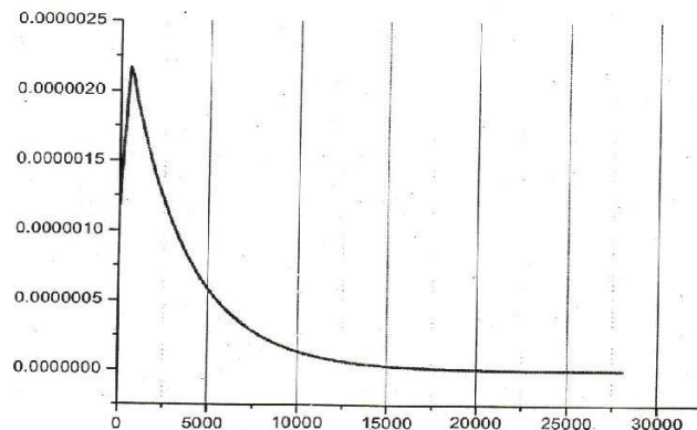
Fig. 12.1. Stiffness Degradation behaviour of Chapsten E-Glass Epoxy laminate Number of Fatigue Cycles at 1.57 RPS for Chapsten E-Glass Epoxy Laminate.
