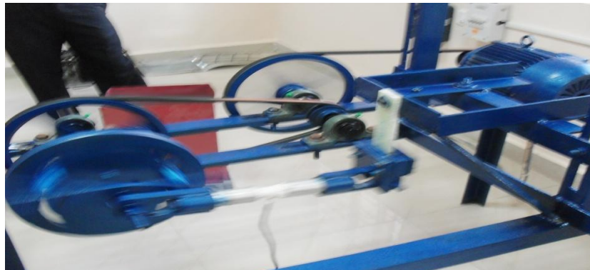
Fig 1. Positioning of composite material in vertical & horizontal directions in Pictorial view of Fatigue Test Rig
