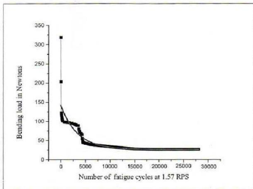
Fig. 12.1. Stiffness Degradation behaviour of Chapsten E-Glass Epoxy laminate Number of Fatigue Cycles at 1.57 RPS for Chapsten E-Glass Epoxy Laminate.
