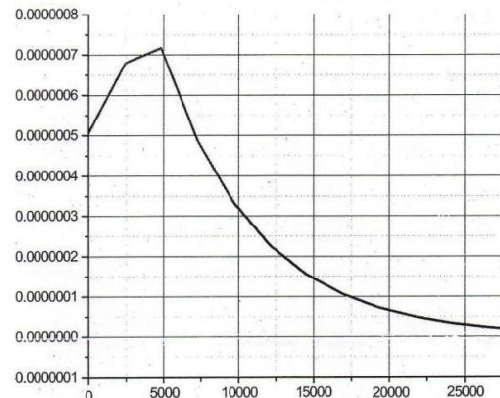
Fig. 11.1 Stiffness Degradation behaviour of Glass Fiber Epoxy laminate Number of Fatigue Cycles at 1.57 RPS for Glass Fiber Epoxy Laminate
