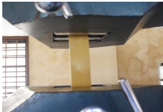
Fig. 9. Tensile Test in Process
