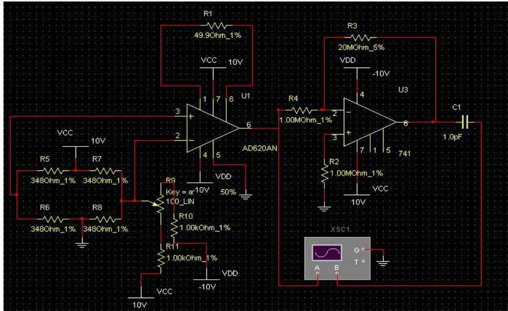
Fig 8.Signal conditioning circuit layout
